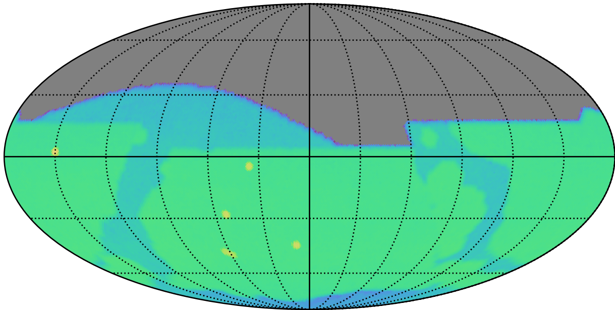
too_elab_r64_d3_giz_v3.4_10yrs r: SurfaceBrightLimit
