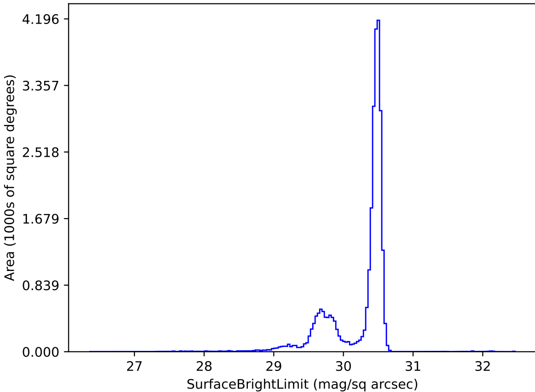
too_elab_r64_d3_giz_v3.4_10yrs r: SurfaceBrightLimit
