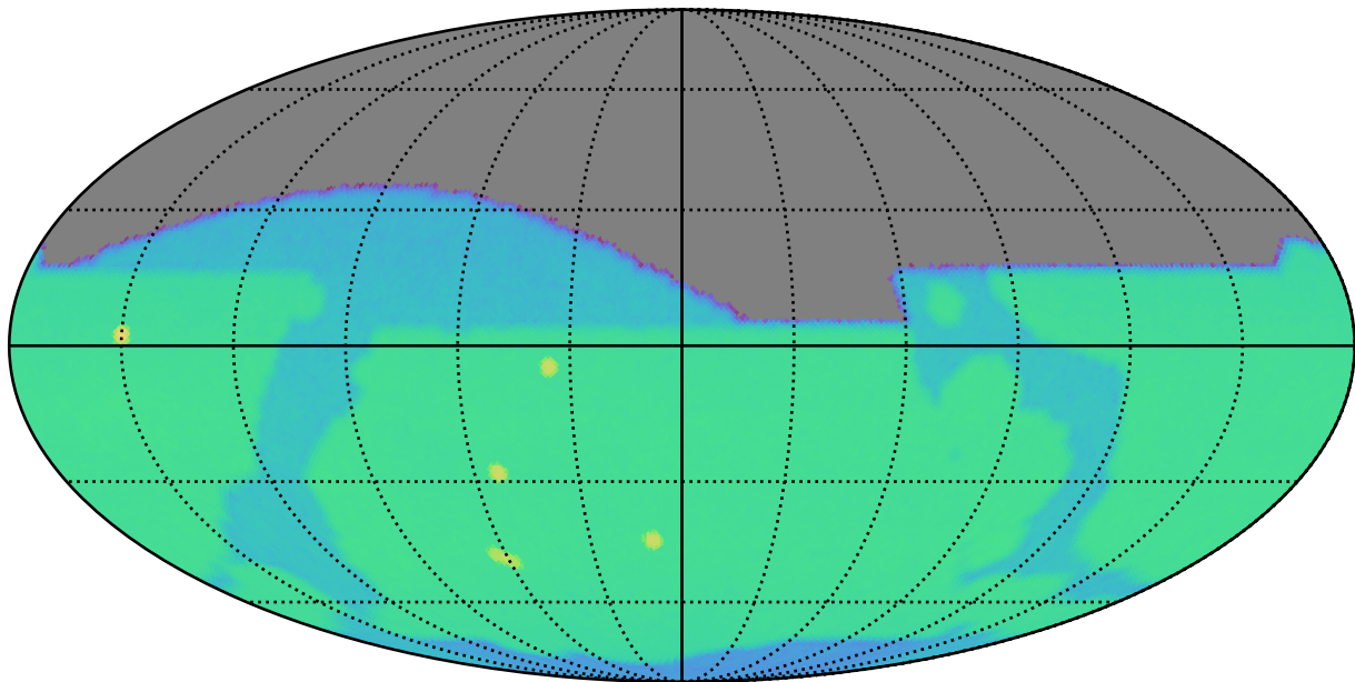
too_elab_r64_d3_giz_v3.4_10yrs i: SurfaceBrightLimit
