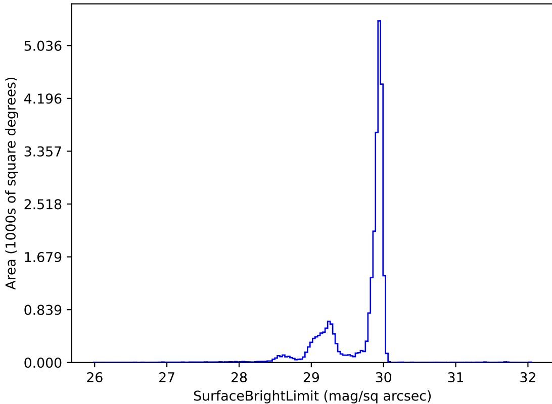
too_elab_r64_d3_giz_v3.4_10yrs i: SurfaceBrightLimit
