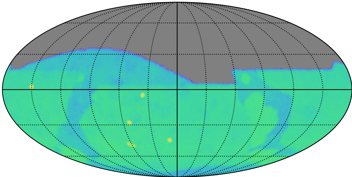
too_elab_r64_d3_giz_v3.4_10yrs g: SurfaceBrightLimit
