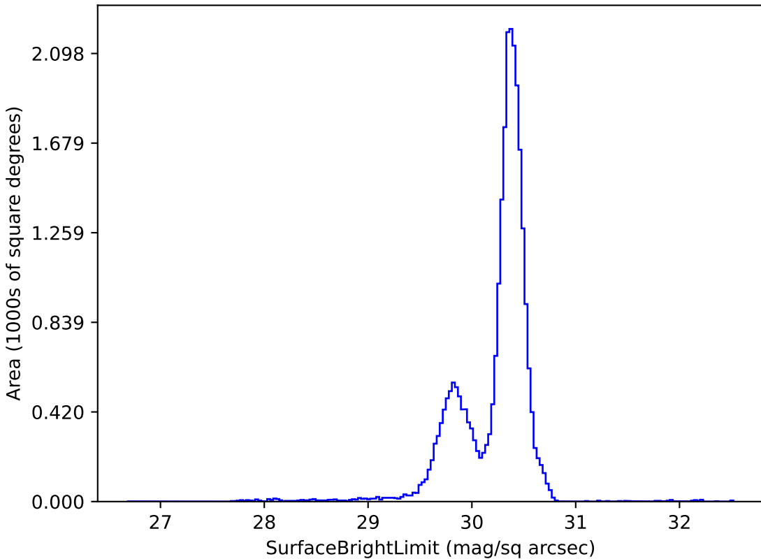
too_elab_r64_d3_giz_v3.4_10yrs g: SurfaceBrightLimit
