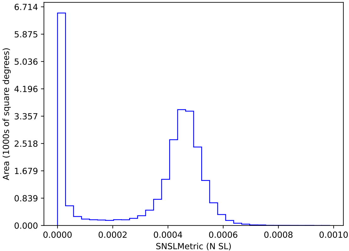
too_elab_r64_d3_giz_v3.4_10yrs : SNSLMetric
