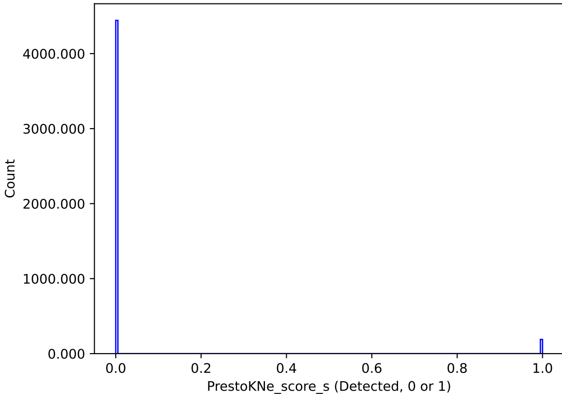
too_elab_r64_d3_giz_v3.4_10yrs : PrestoKNe_score_s
