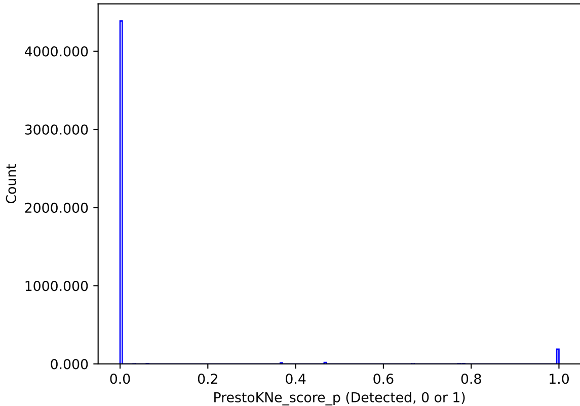
too_elab_r64_d3_giz_v3.4_10yrs : PrestoKNe_score_p
