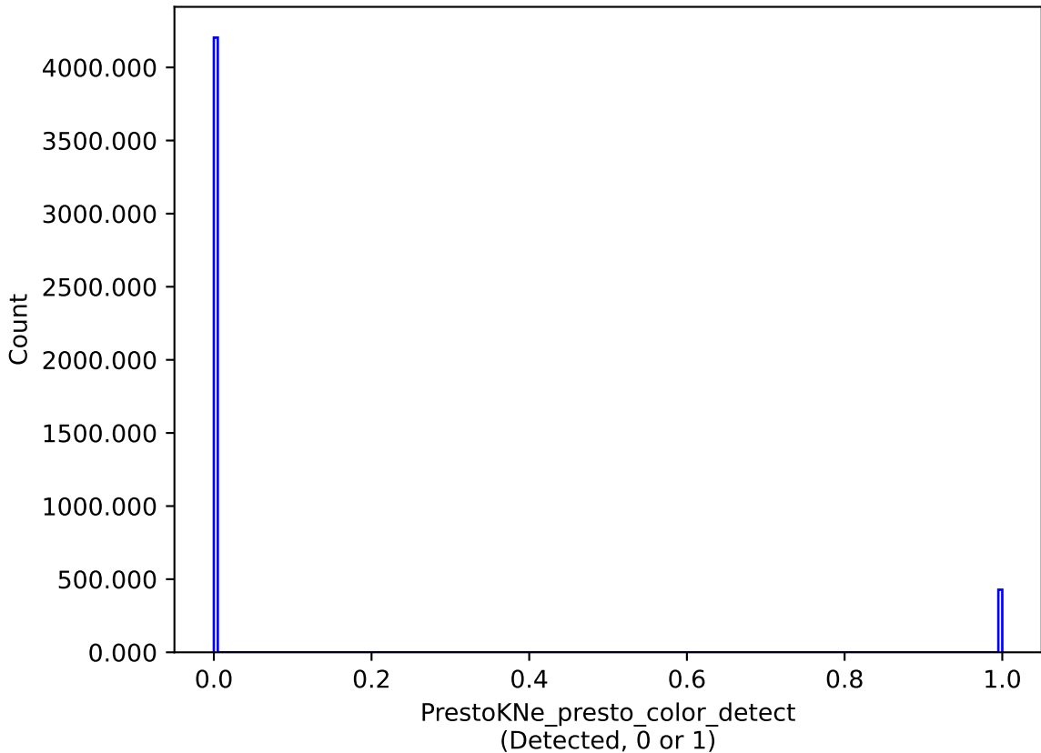
too_elab_r64_d3_giz_v3.4_10yrs : PrestoKNe_presto_color_detect
