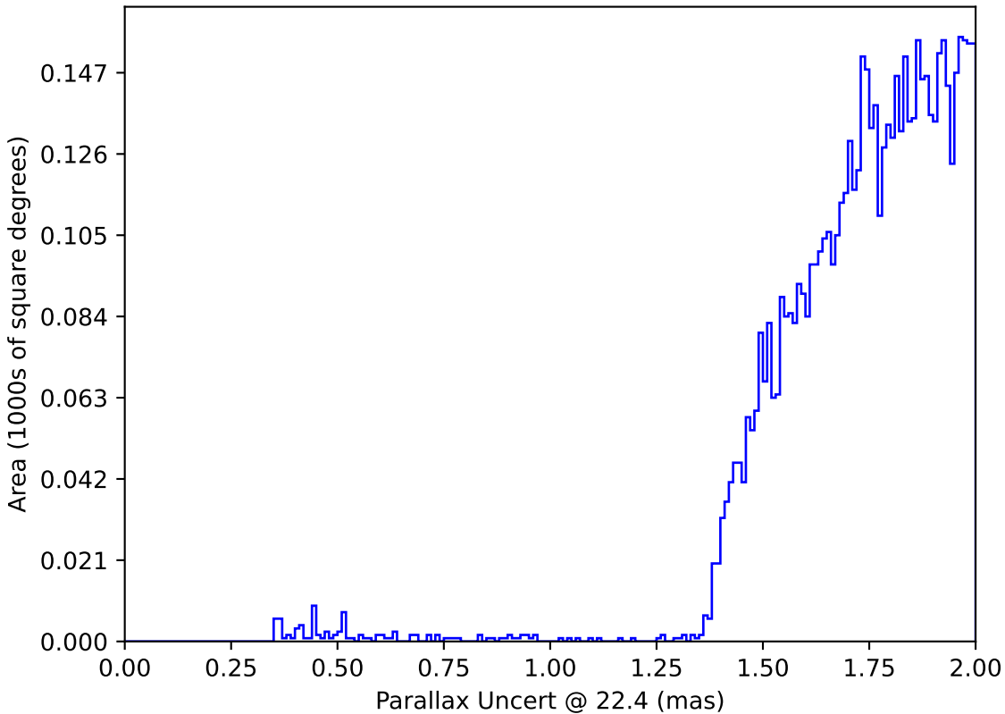
too_elab_r64_d3_giz_v3.4_10yrs : Parallax Uncert @ 22.4
