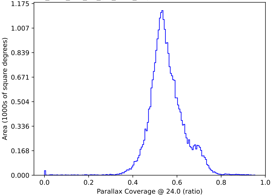
too_elab_r64_d3_giz_v3.4_10yrs : Parallax Coverage @ 24.0
