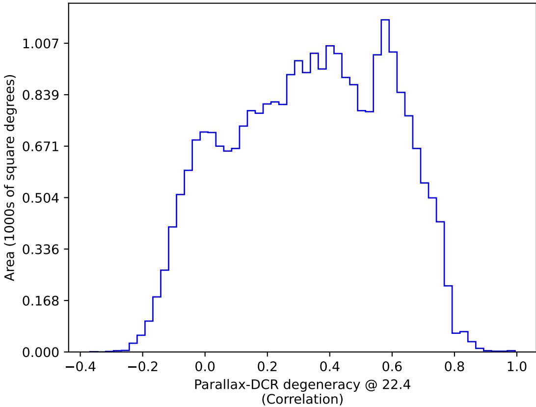
too_elab_r64_d3_giz_v3.4_10yrs : Parallax-DCR degeneracy @ 22.4
