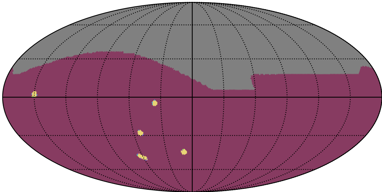
too_elab_r64_d3_giz_v3.4_10yrs : NumberOfQuickRevisits
