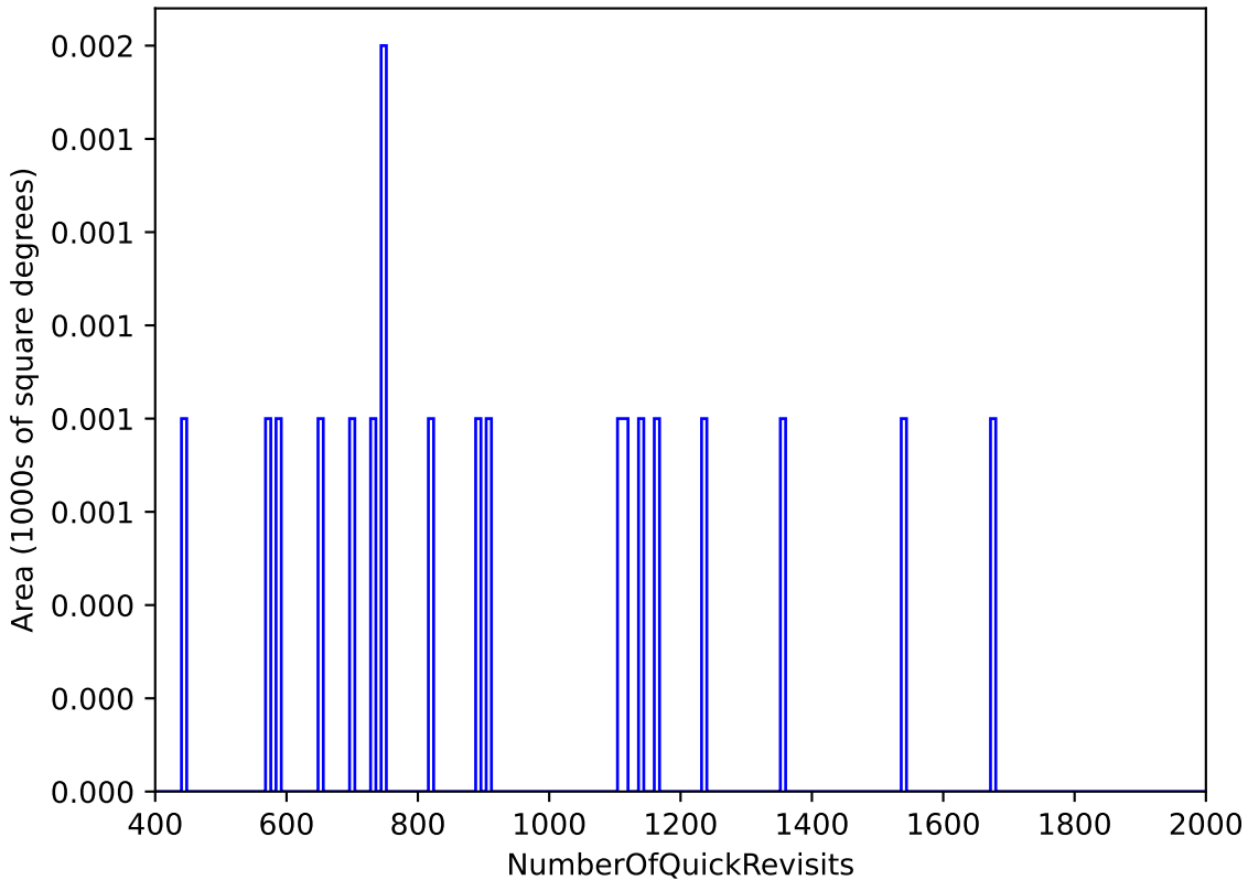
too_elab_r64_d3_giz_v3.4_10yrs : NumberOfQuickRevisits
