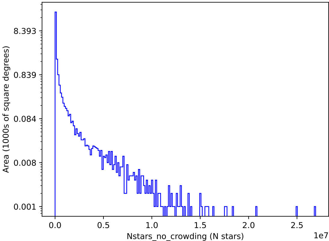
too_elab_r64_d3_giz_v3.4_10yrs z: Nstars_no_crowding
