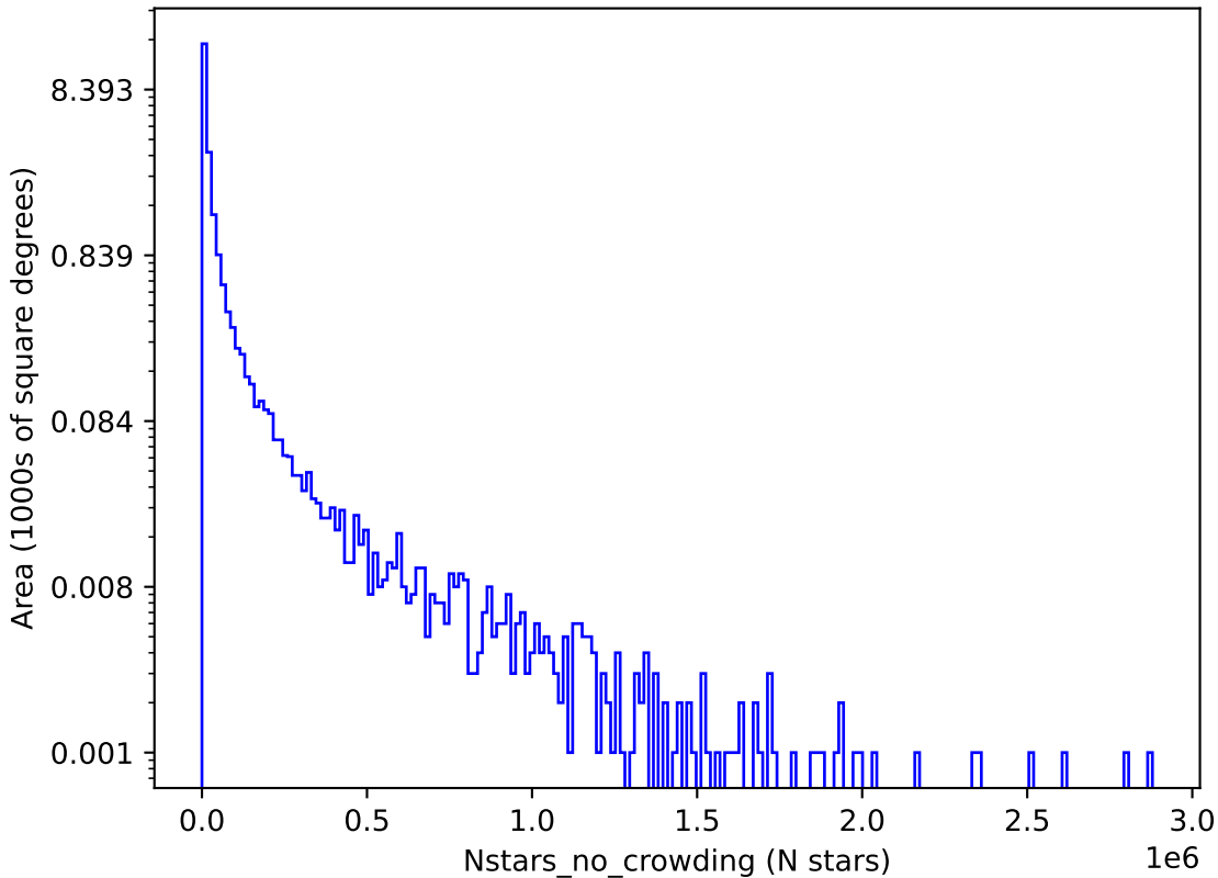
too_elab_r64_d3_giz_v3.4_10yrs u: Nstars_no_crowding
