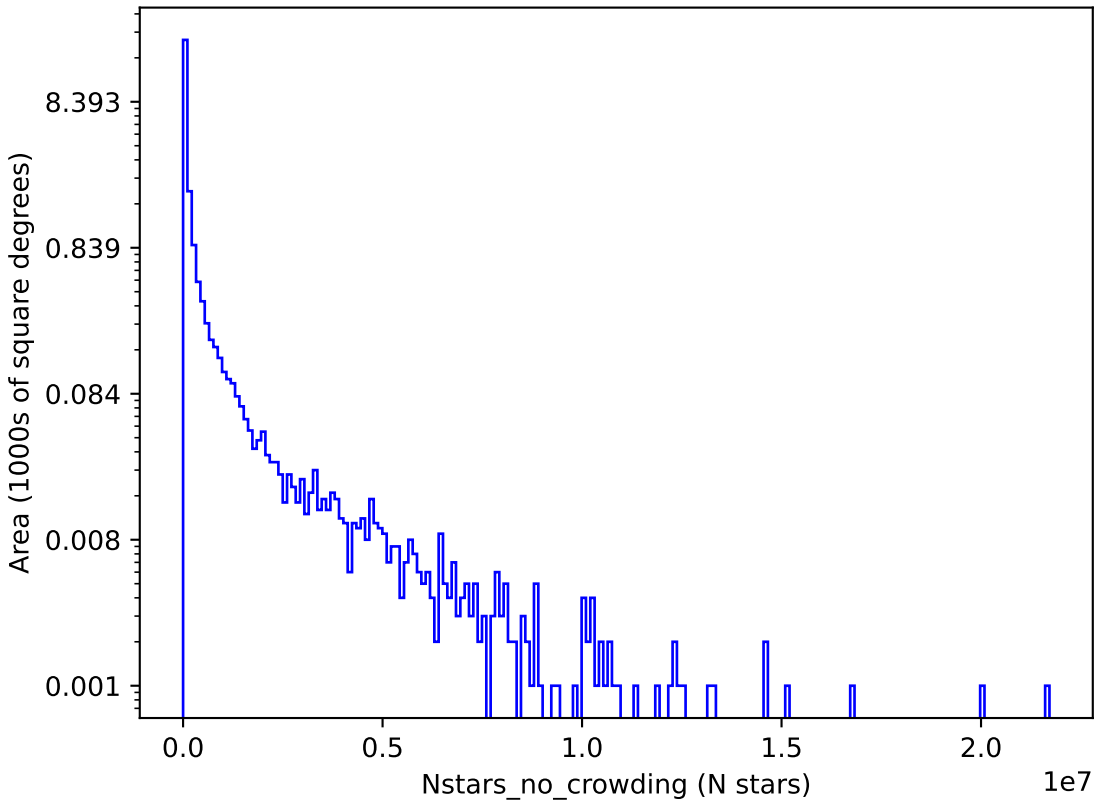
too_elab_r64_d3_giz_v3.4_10yrs r: Nstars_no_crowding
