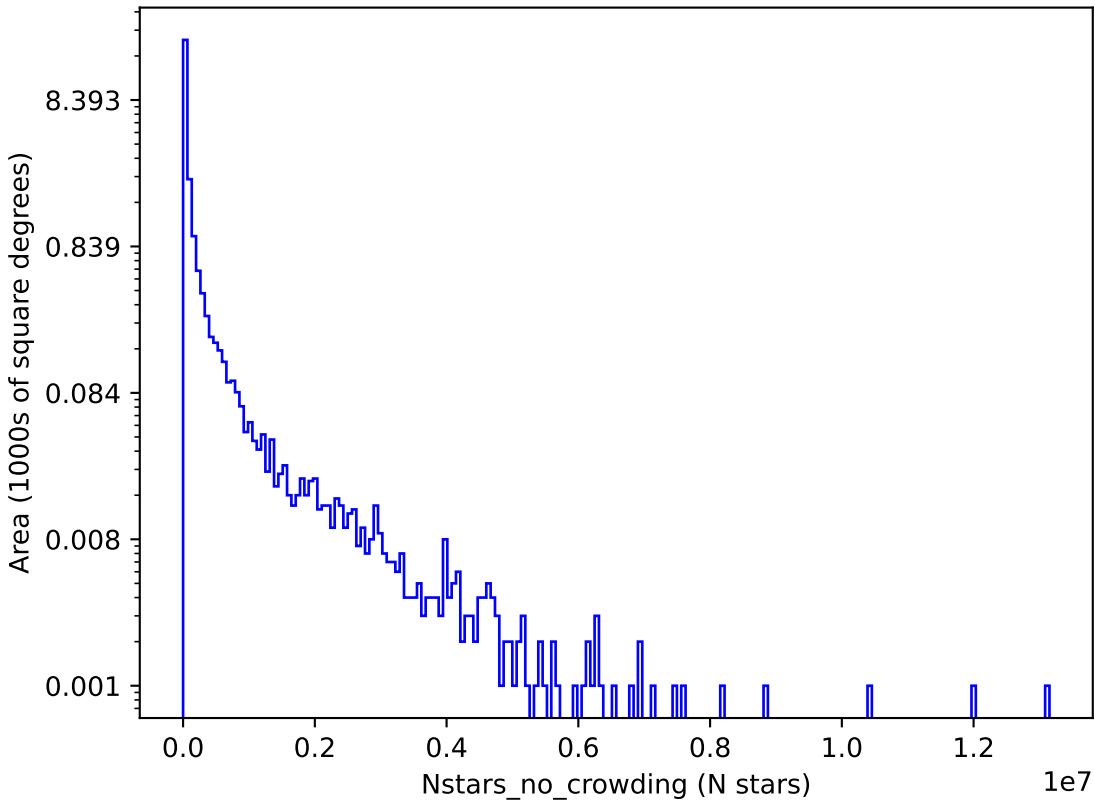
too_elab_r64_d3_giz_v3.4_10yrs g: Nstars_no_crowding
