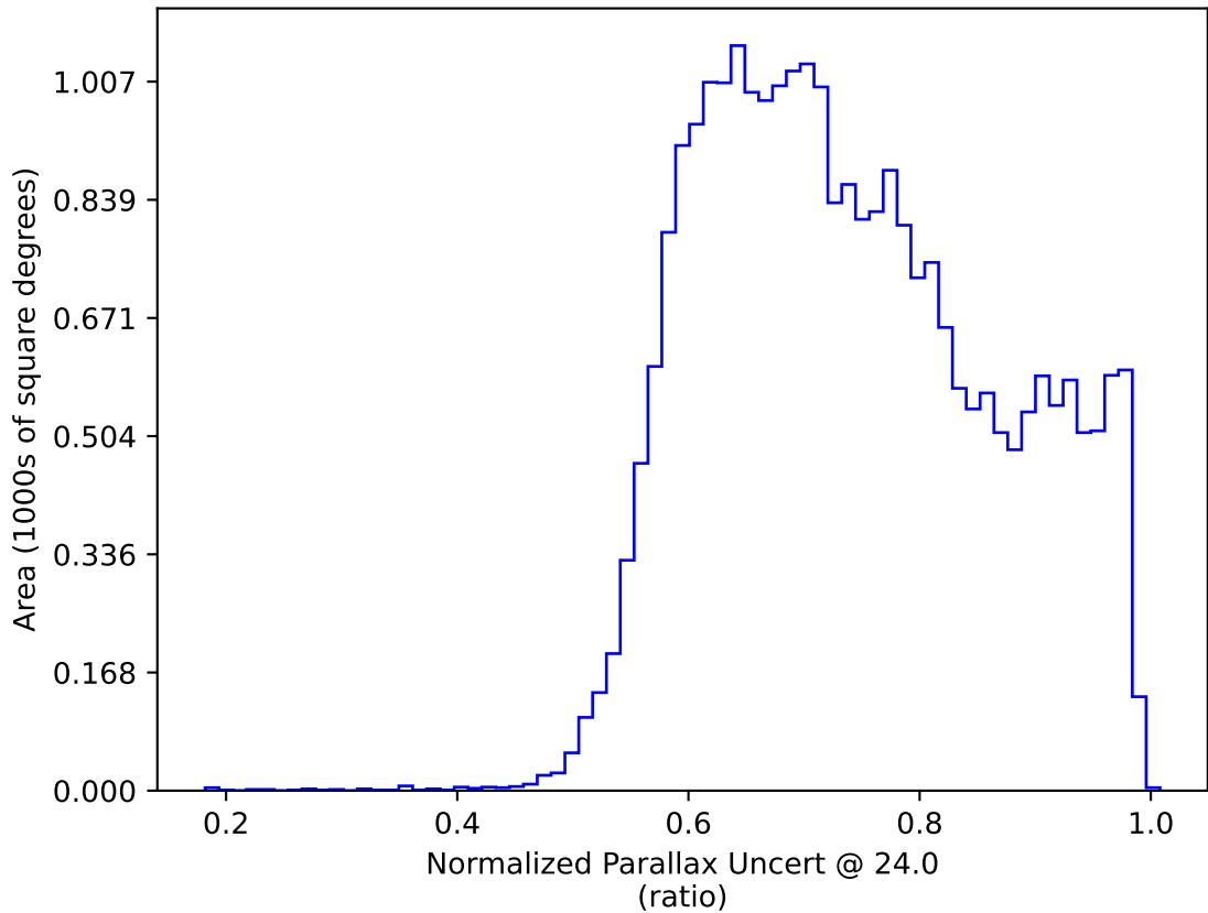
too_elab_r64_d3_giz_v3.4_10yrs : Normalized Parallax Uncert @ 24.0
