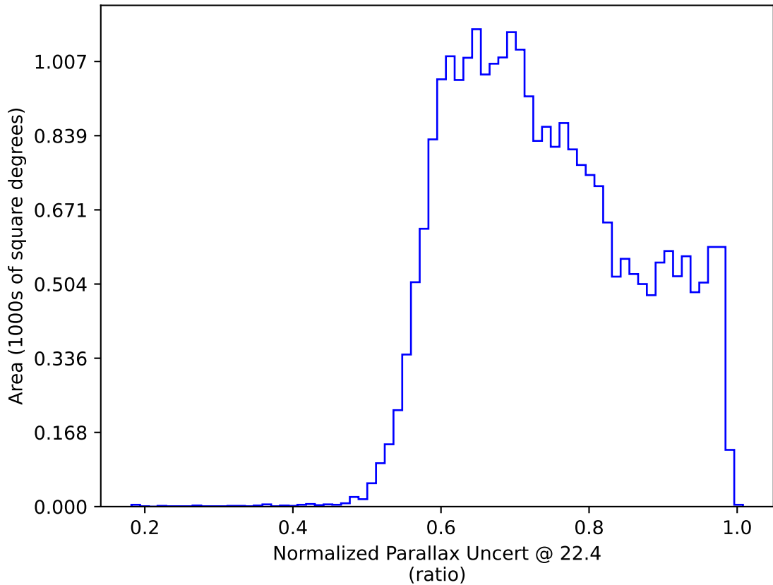
too_elab_r64_d3_giz_v3.4_10yrs : Normalized Parallax Uncert @ 22.4
