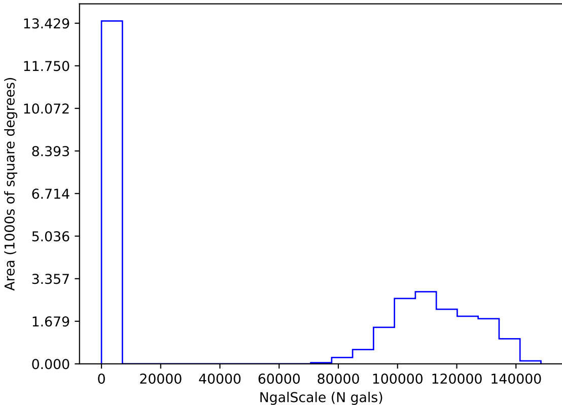
too_elab_r64_d3_giz_v3.4_10yrs i: NgalScale
