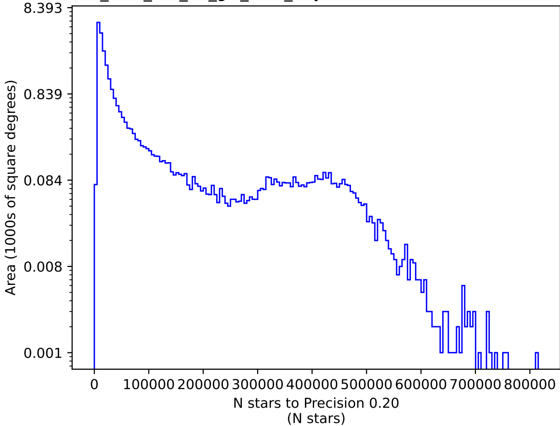
too_elab_r64_d3_giz_v3.4_10yrs i: N stars to Precision 0.20
