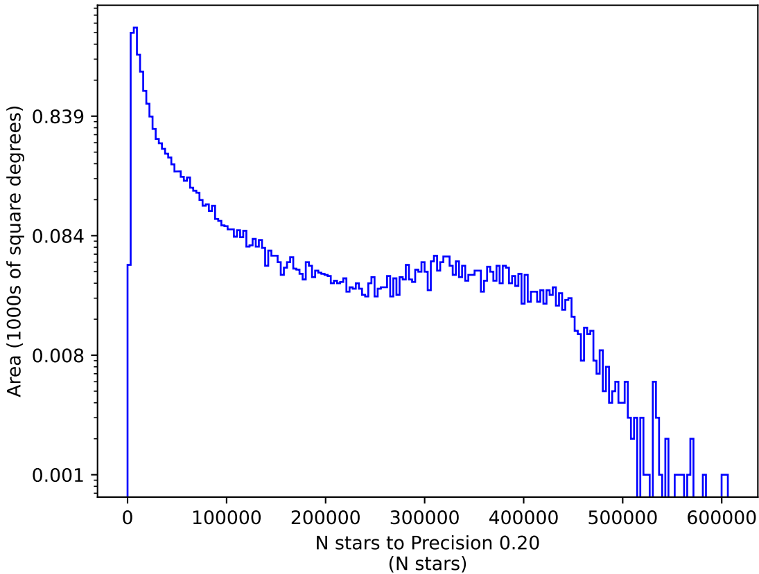
too_elab_r64_d3_giz_v3.4_10yrs g: N stars to Precision 0.20
