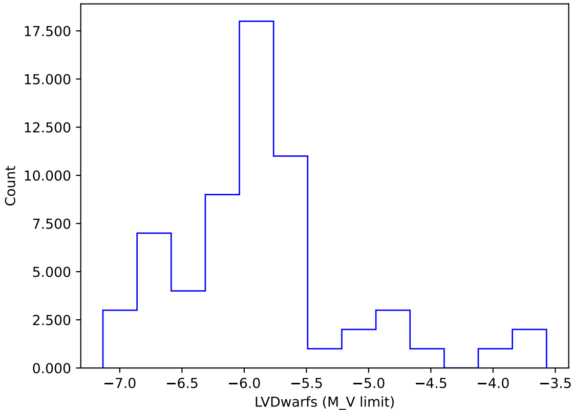
too_elab_r64_d3_giz_v3.4_10yrs gi: LVDwarfs
