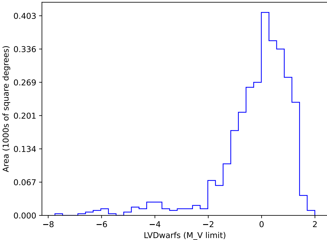
too_elab_r64_d3_giz_v3.4_10yrs gi SCP: LVDwarfs
