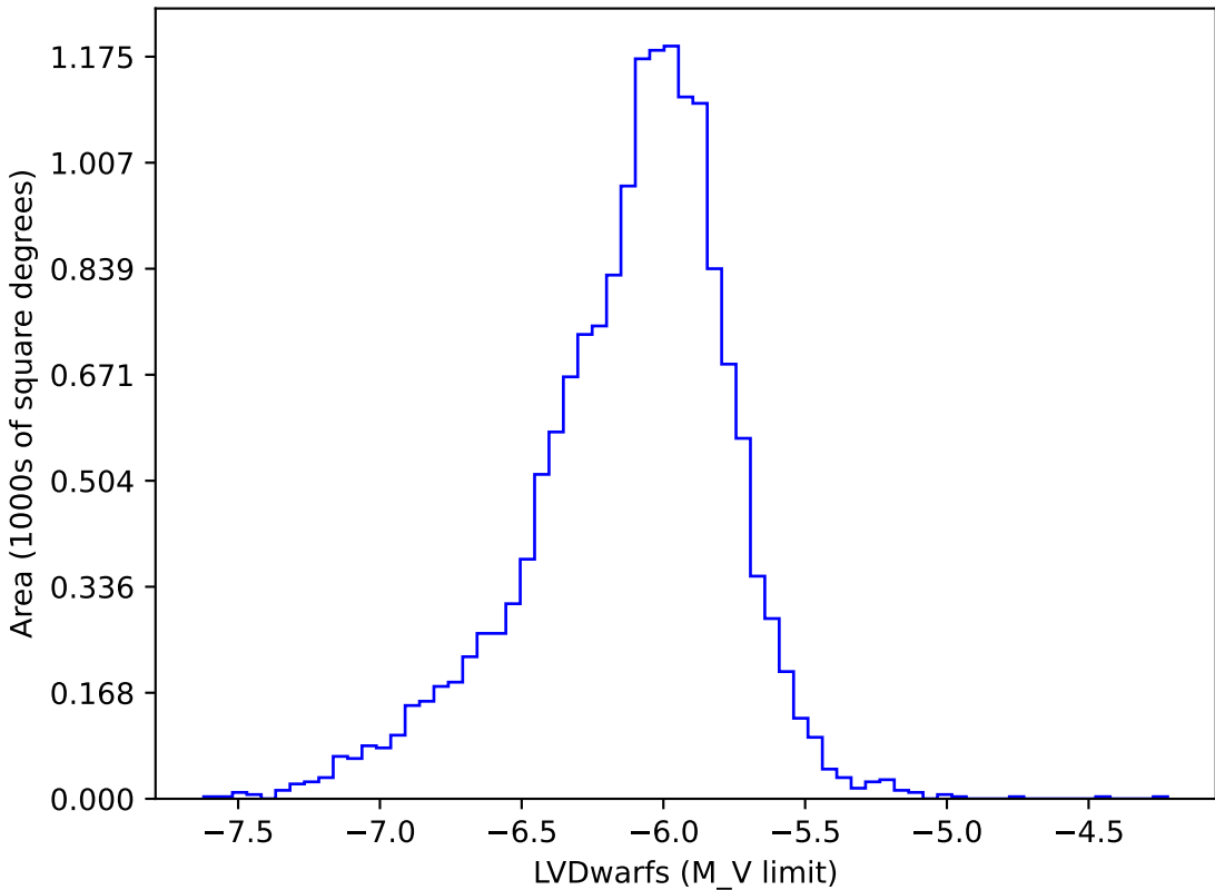
too_elab_r64_d3_giz_v3.4_10yrs gi: LVDwarfs
