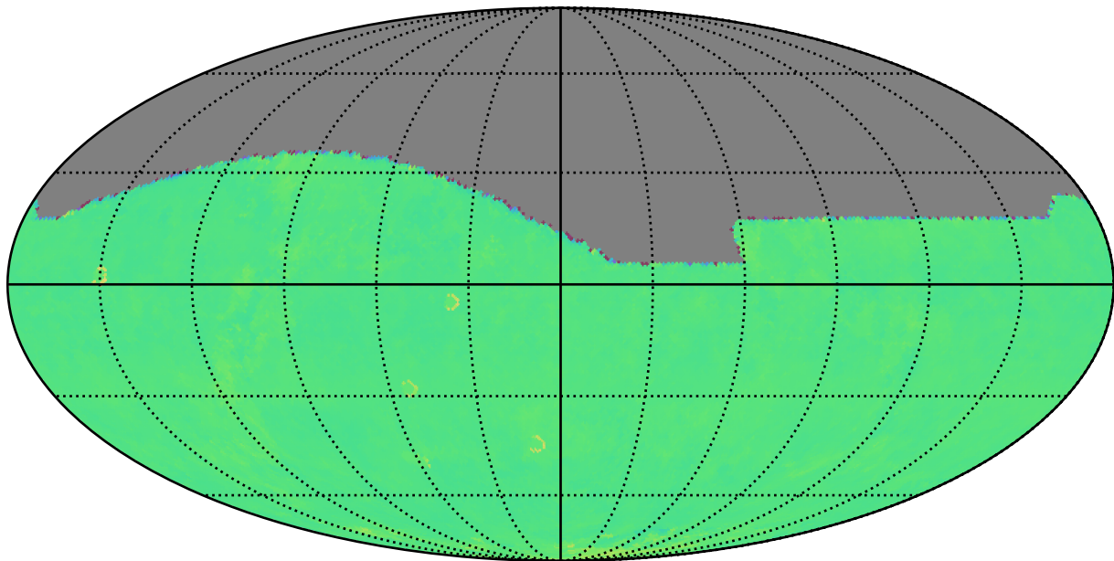
too_elab_r64_d3_giz_v3.4_10yrs r: Kuiper rotTelPos
