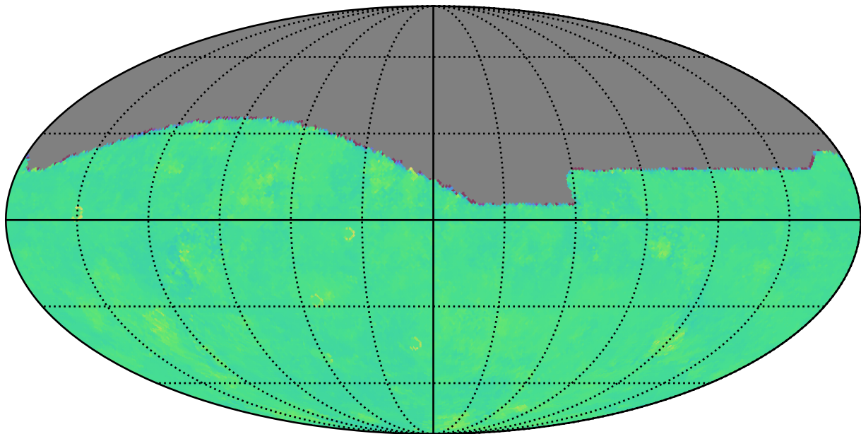
too_elab_r64_d3_giz_v3.4_10yrs g: Kuiper rotTelPos
