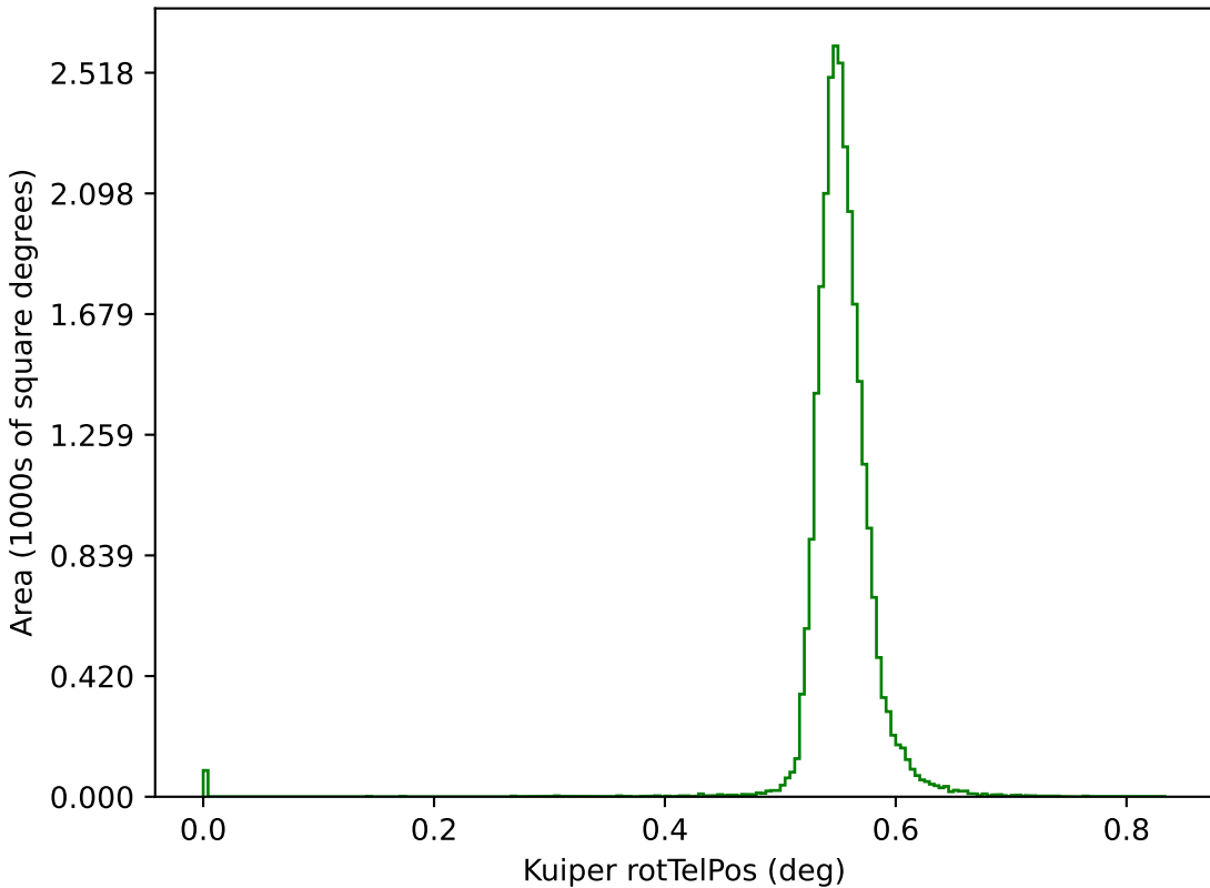
too_elab_r64_d3_giz_v3.4_10yrs g: Kuiper rotTelPos
