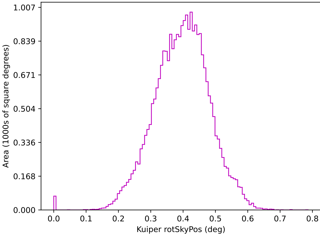
too_elab_r64_d3_giz_v3.4_10yrs z: Kuiper rotSkyPos
