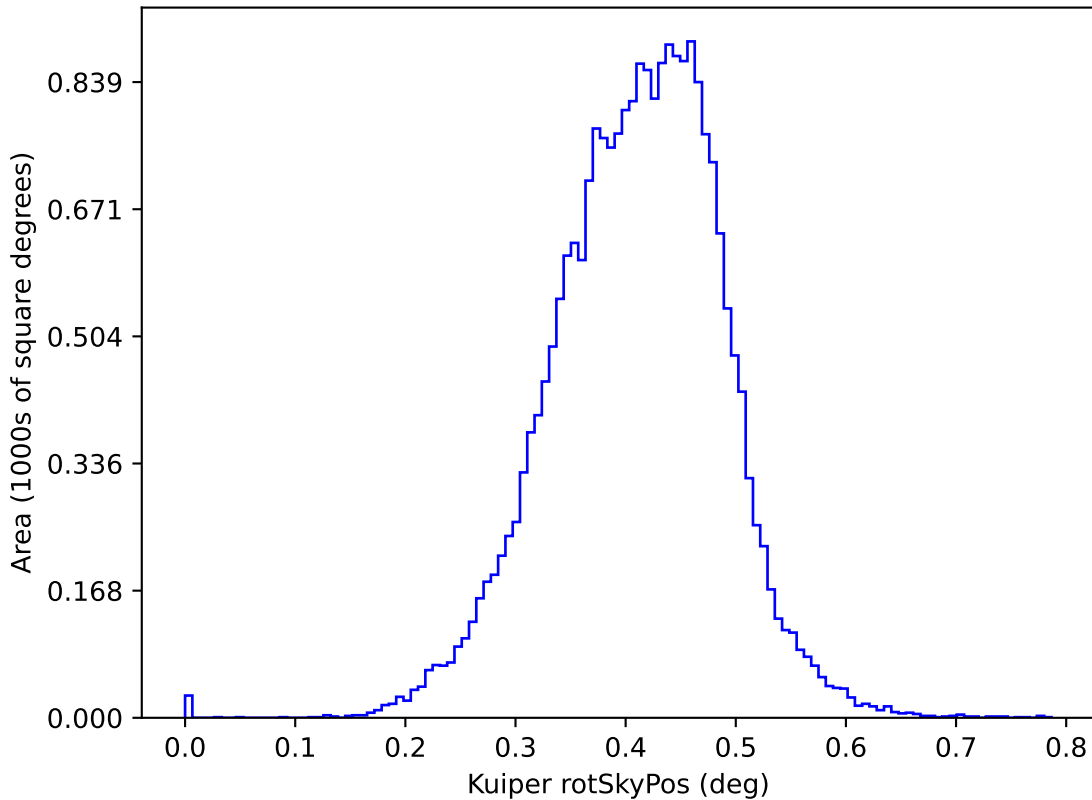
too_elab_r64_d3_giz_v3.4_10yrs y: Kuiper rotSkyPos
