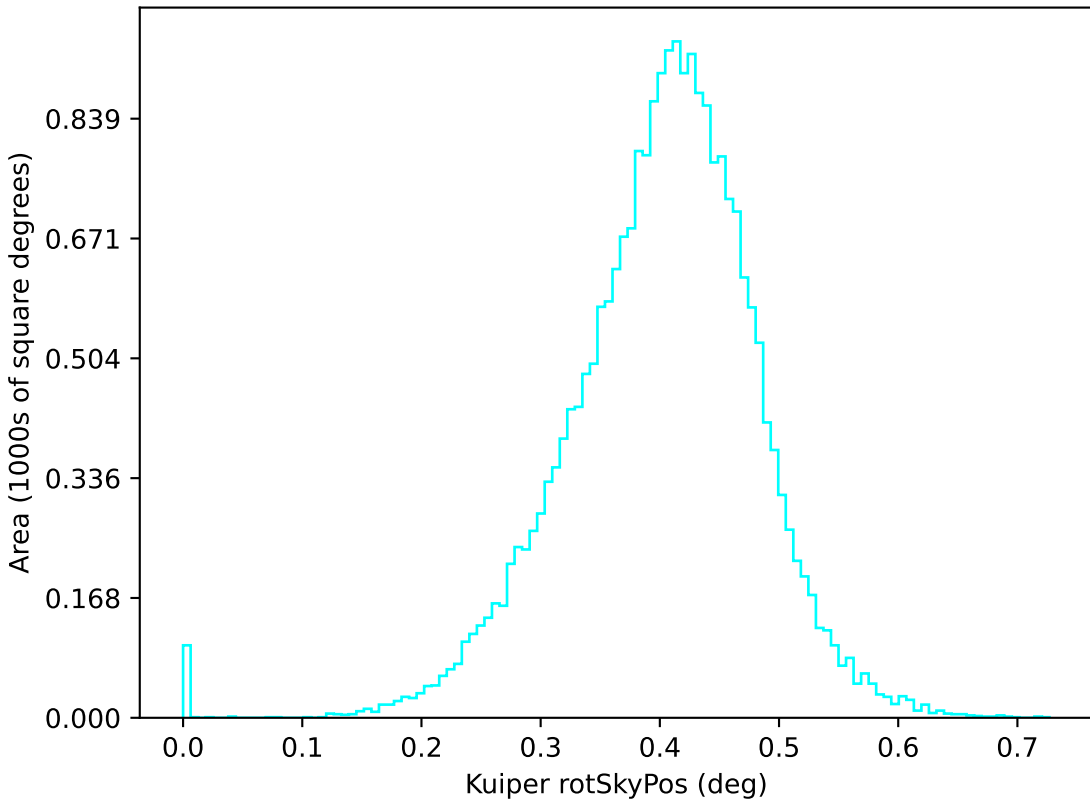
too_elab_r64_d3_giz_v3.4_10yrs u: Kuiper rotSkyPos
