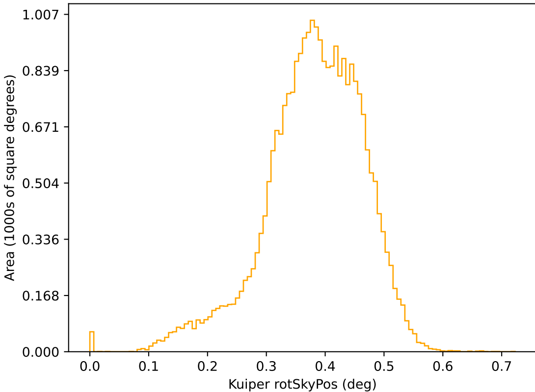
too_elab_r64_d3_giz_v3.4_10yrs r: Kuiper rotSkyPos
