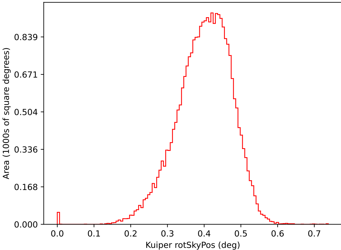
too_elab_r64_d3_giz_v3.4_10yrs i: Kuiper rotSkyPos
