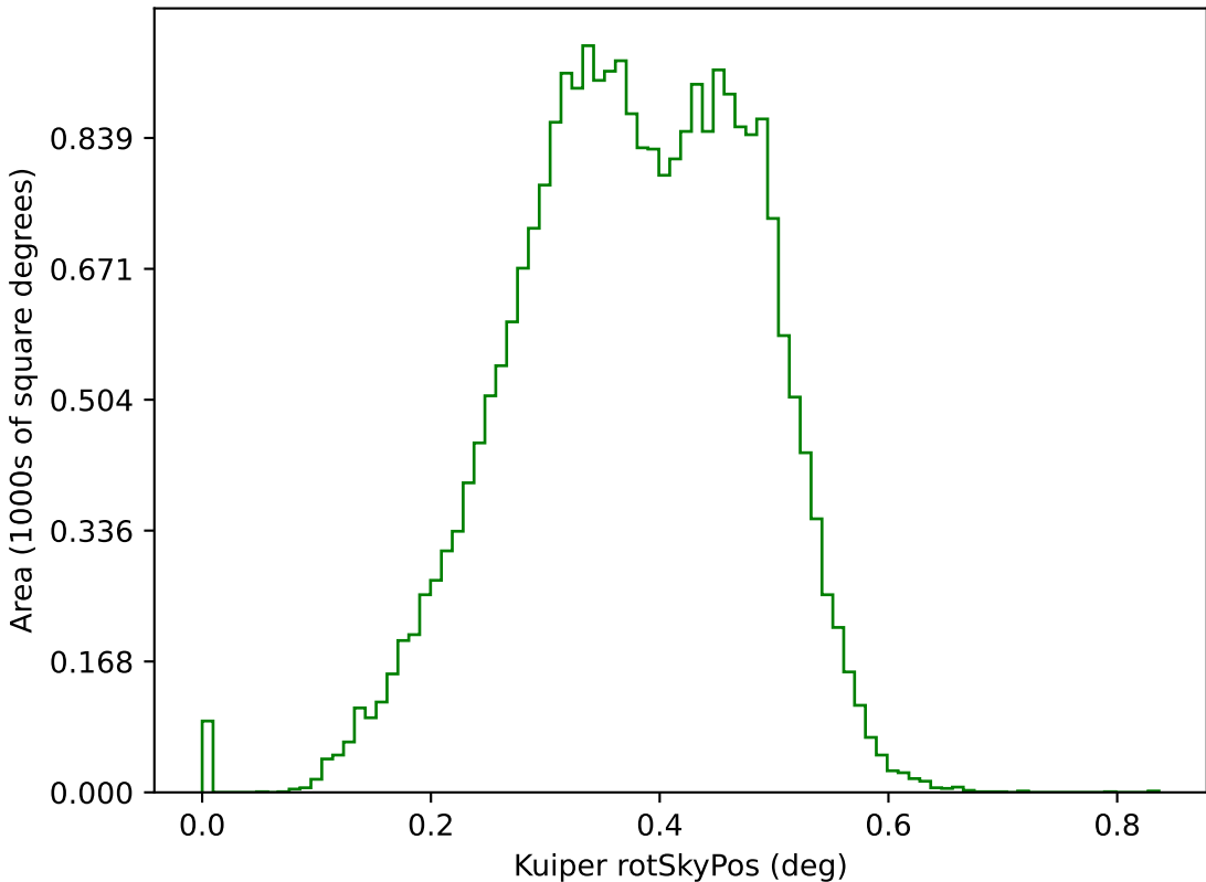
too_elab_r64_d3_giz_v3.4_10yrs g: Kuiper rotSkyPos
