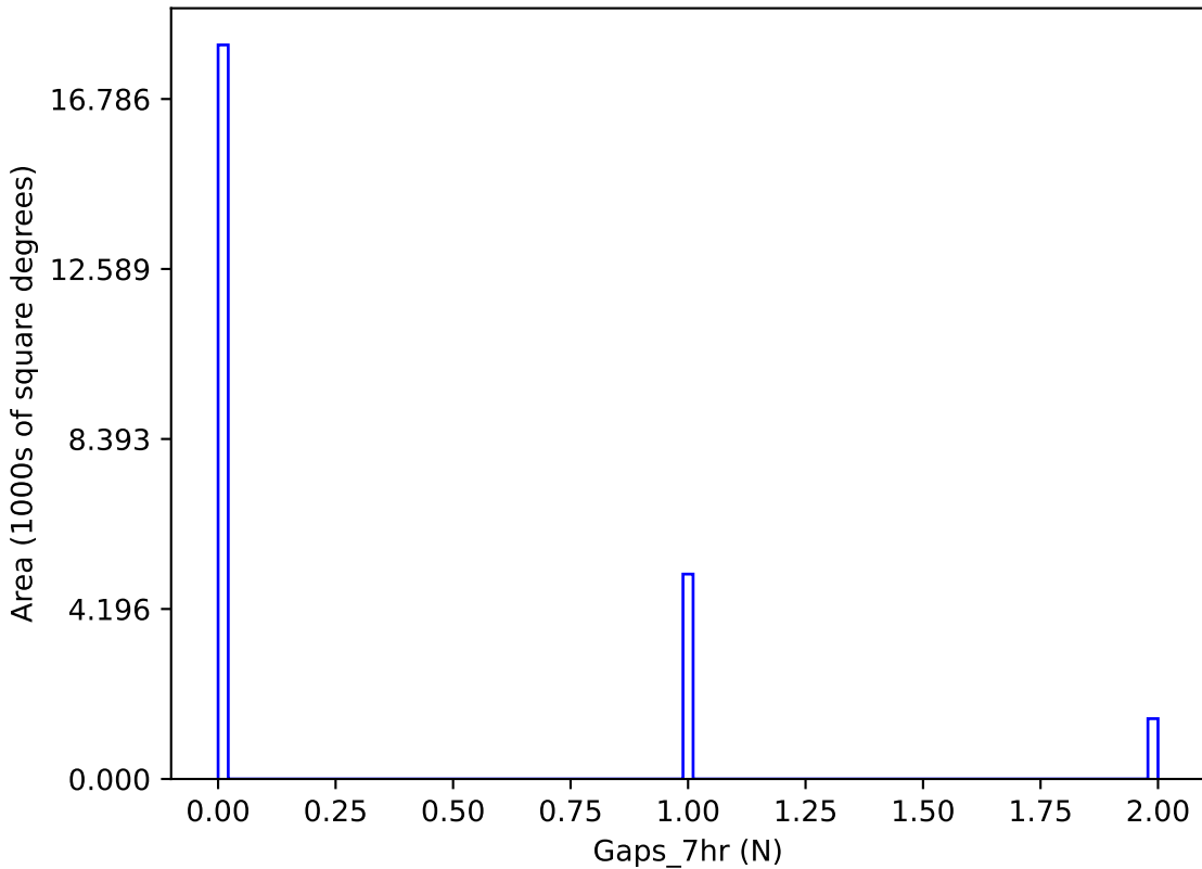
too_elab_r64_d3_giz_v3.4_10yrs y band: Gaps_7hr
