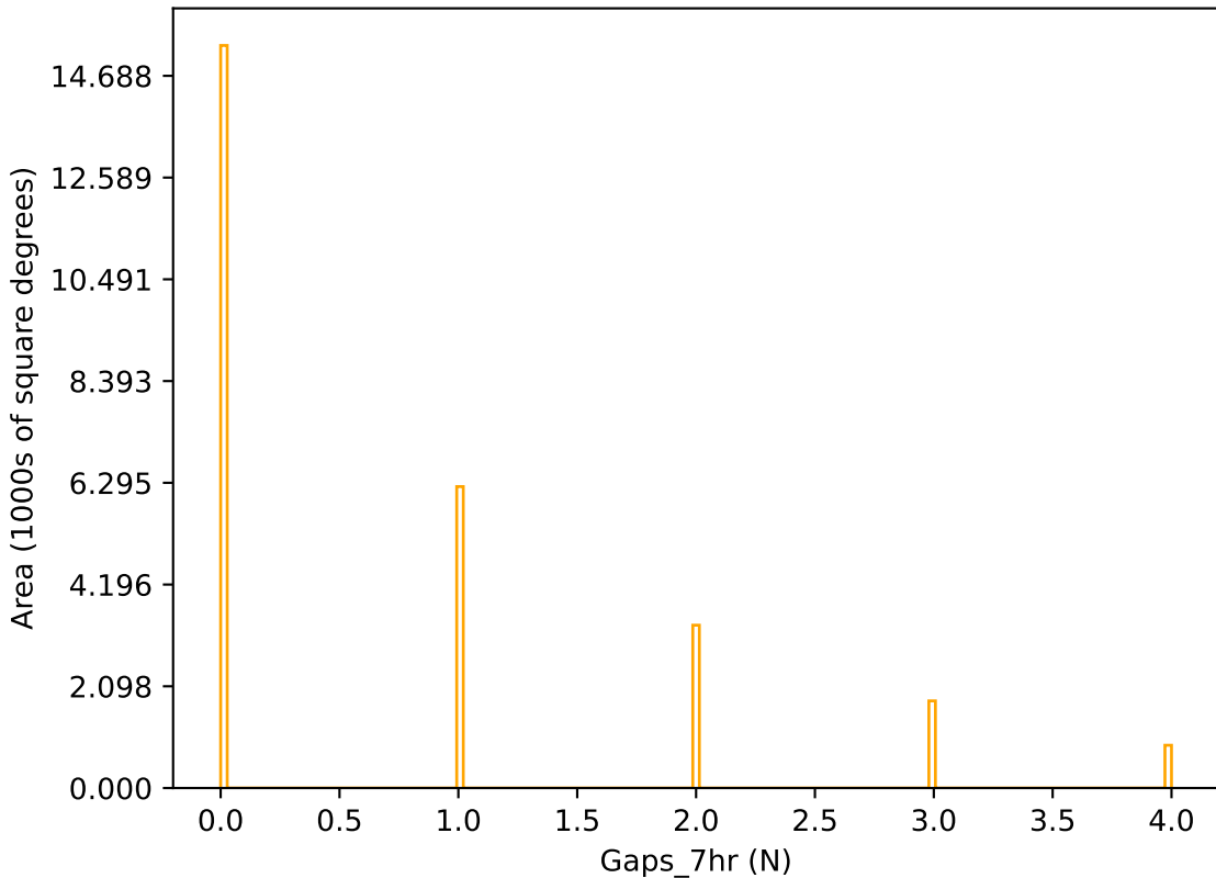
too_elab_r64_d3_giz_v3.4_10yrs r band: Gaps_7hr
