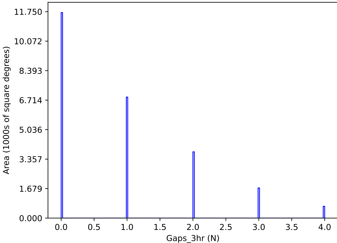
too_elab_r64_d3_giz_v3.4_10yrs y band: Gaps_3hr
