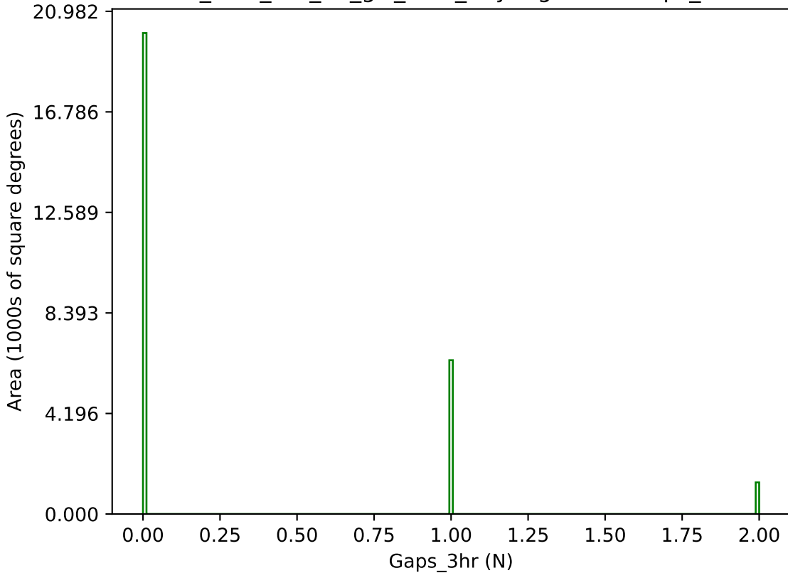
too_elab_r64_d3_giz_v3.4_10yrs g band: Gaps_3hr
