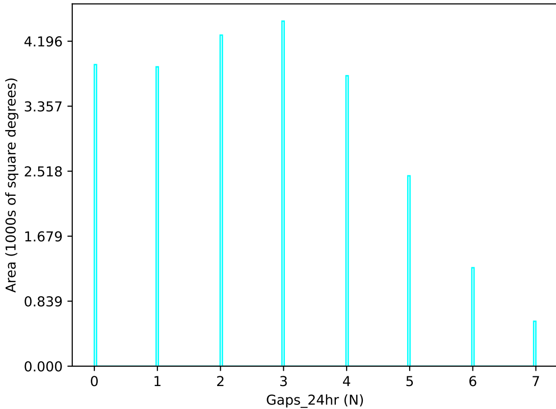
too_elab_r64_d3_giz_v3.4_10yrs u band: Gaps_24hr
