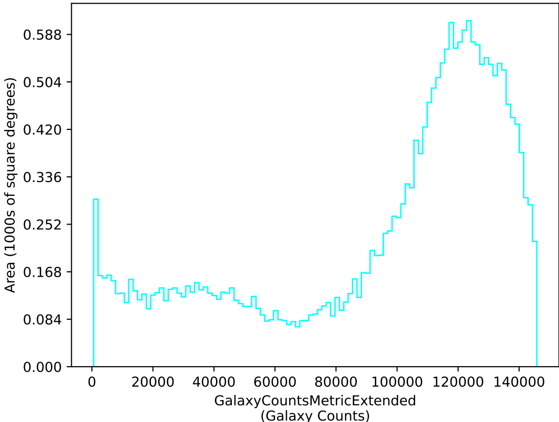
too_elab_r64_d3_giz_v3.4_10yrs u: GalaxyCountsMetricExtended
