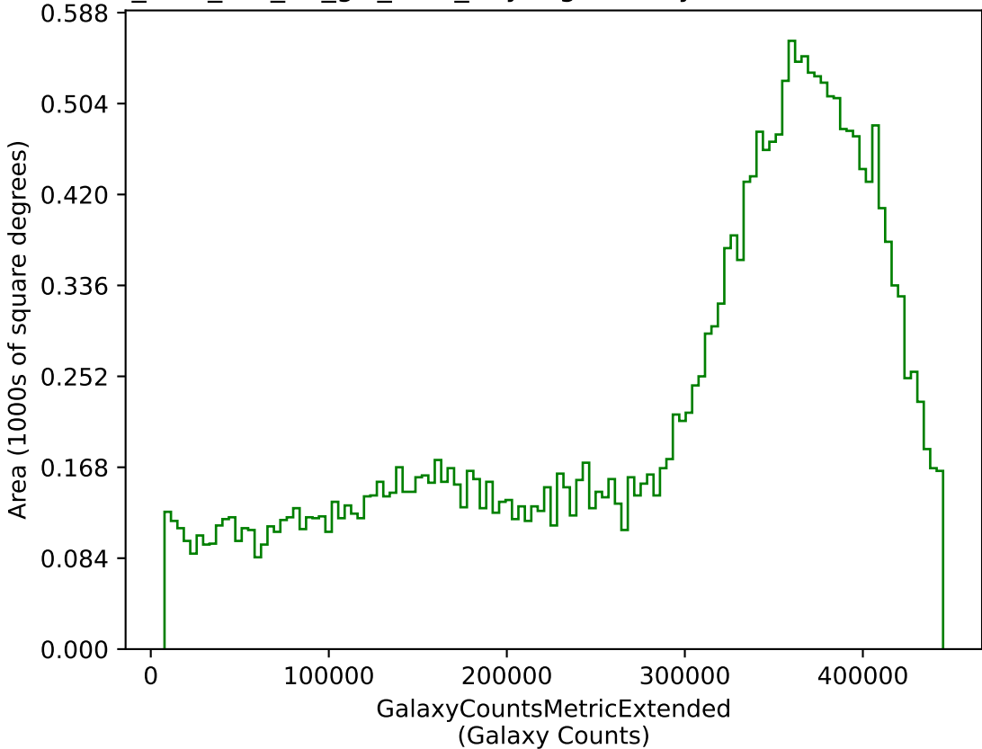
too_elab_r64_d3_giz_v3.4_10yrs g: GalaxyCountsMetricExtended
