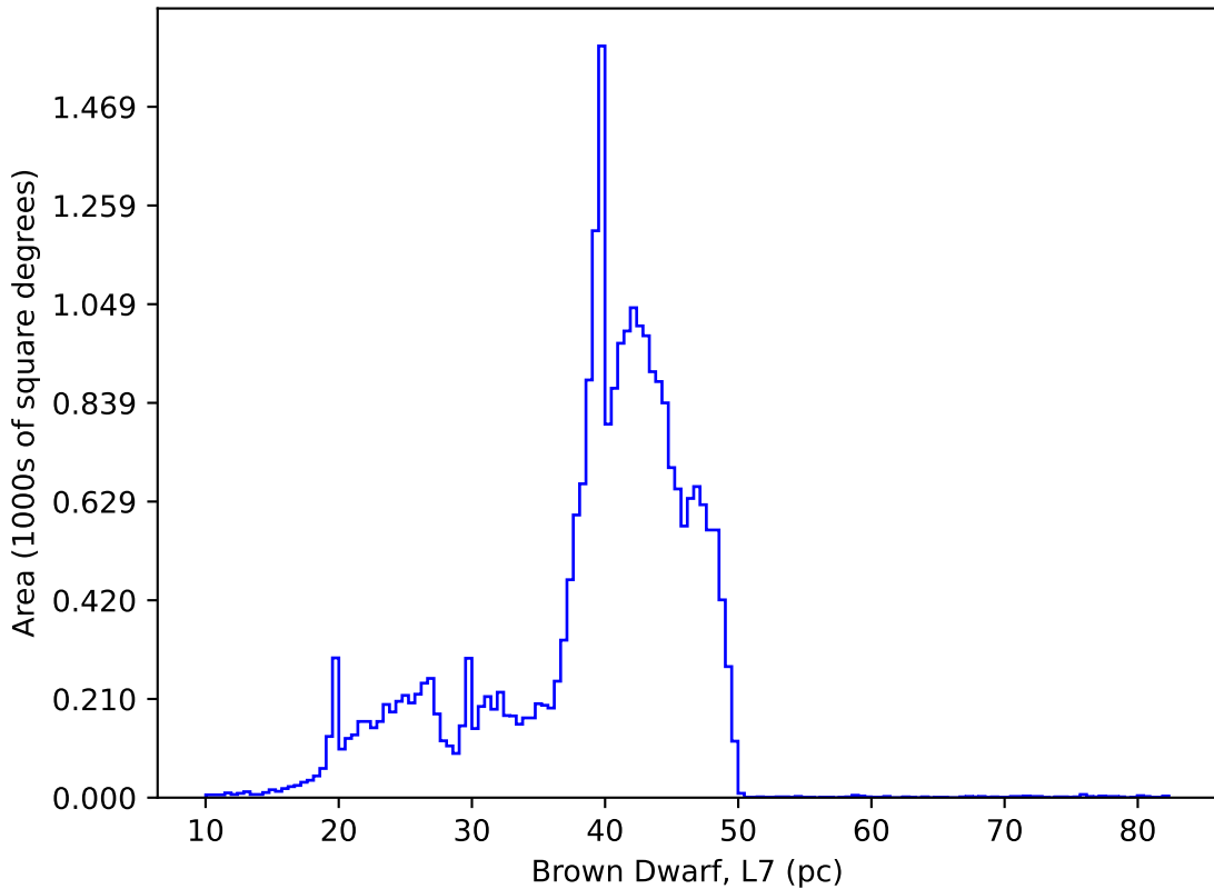
too_elab_r64_d3_giz_v3.4_10yrs : Brown Dwarf, L7
