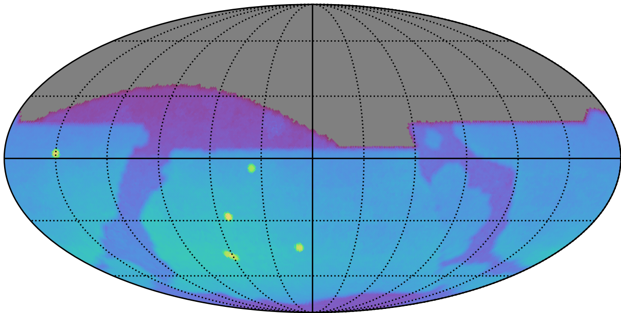
too_elab_r64_d3_giz_v3.4_10yrs : Brown Dwarf, L4
