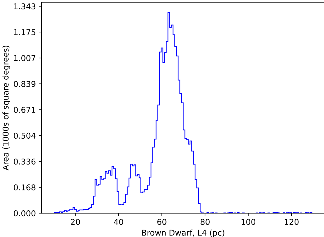
too_elab_r64_d3_giz_v3.4_10yrs : Brown Dwarf, L4
