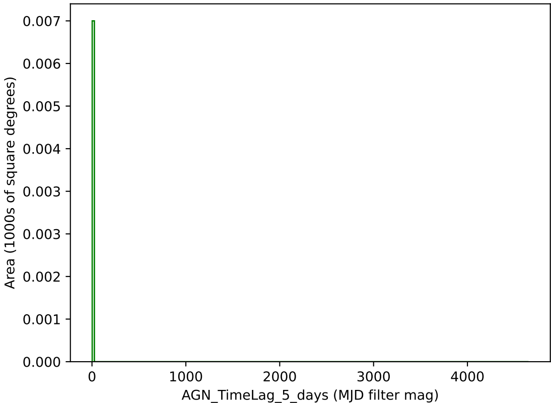
too_elab_r64_d3_giz_v3.4_10yrs g band: AGN_TimeLag_5_days
