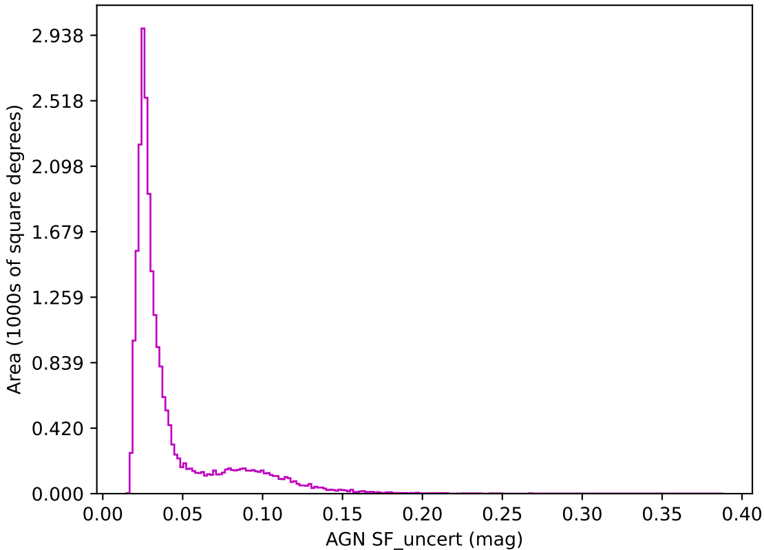
too_elab_r64_d3_giz_v3.4_10yrs z band: AGN SF_uncert
