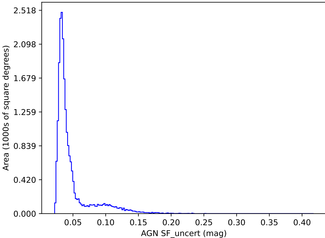
too_elab_r64_d3_giz_v3.4_10yrs y band: AGN SF_uncert
