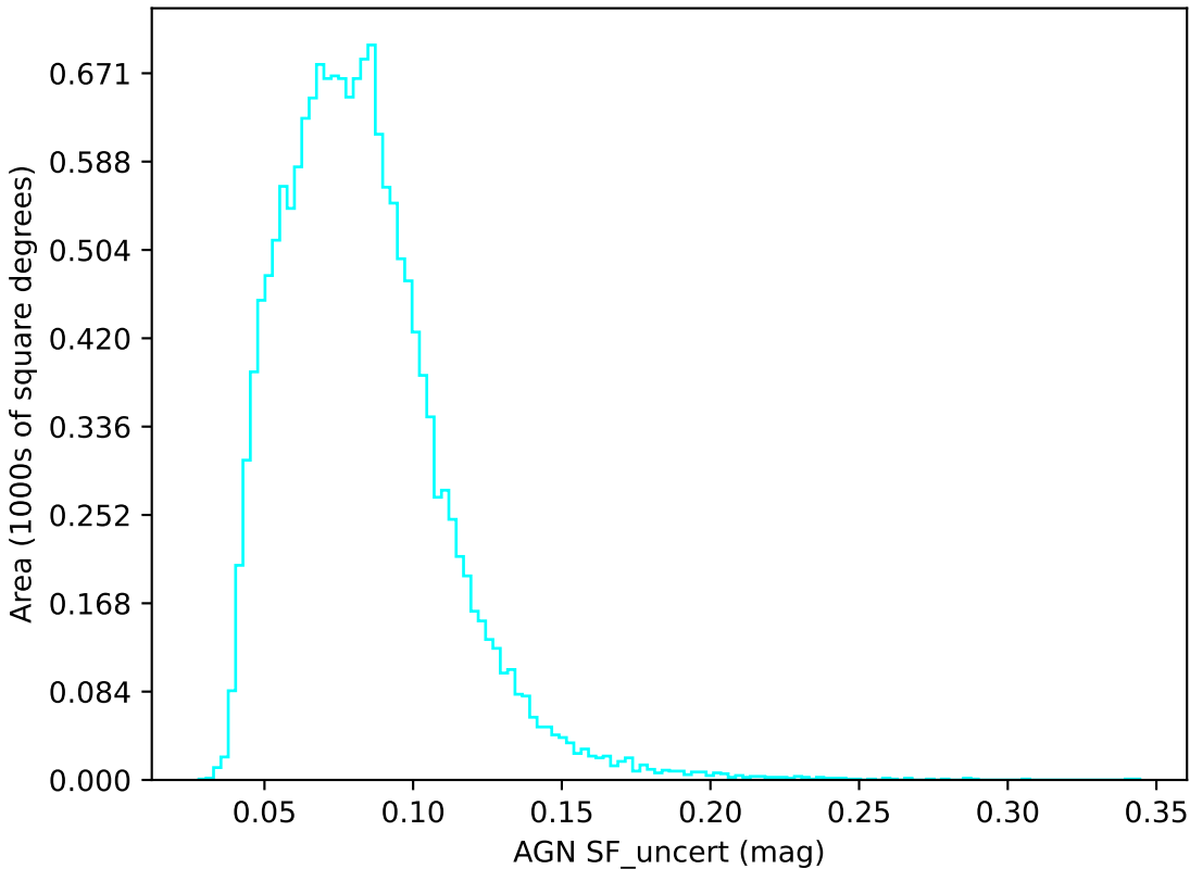
too_elab_r64_d3_giz_v3.4_10yrs u band: AGN SF_uncert
